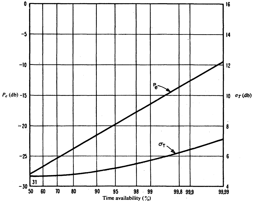
FIGURE 31 Expected values of P_e and their standard deviations \sigma_T
