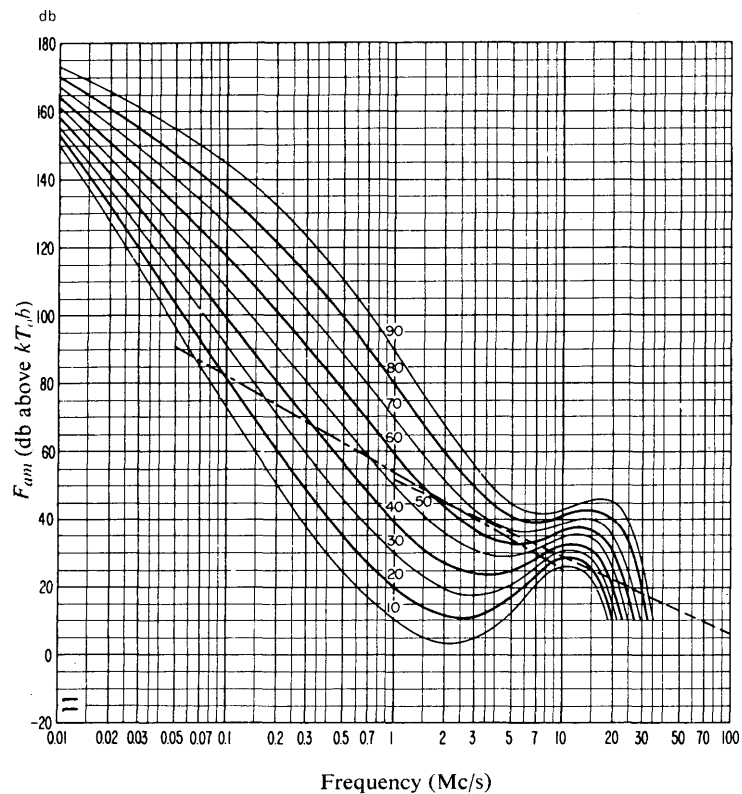
FIGURE 11B Variation of radio noise with frequency (Spring; 1200–1600 h.)
