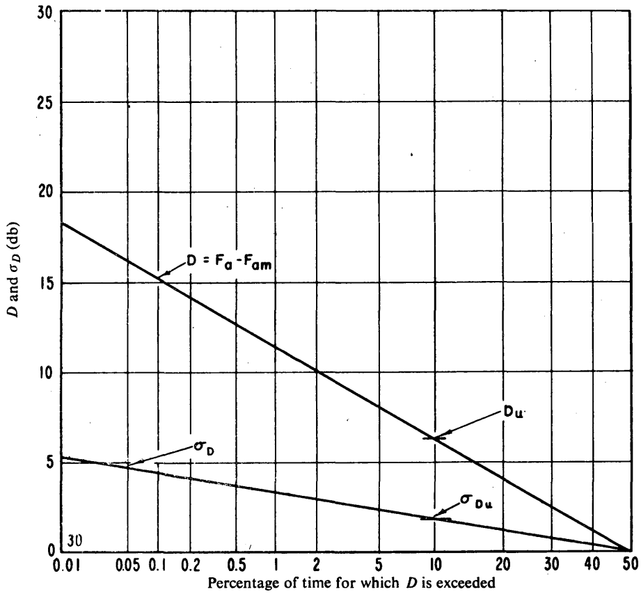
FIGURE 30 Expected values of D and their standard deviations \sigma_D Summer season, 2000–2400 h. Frequency: 50 kc/s
