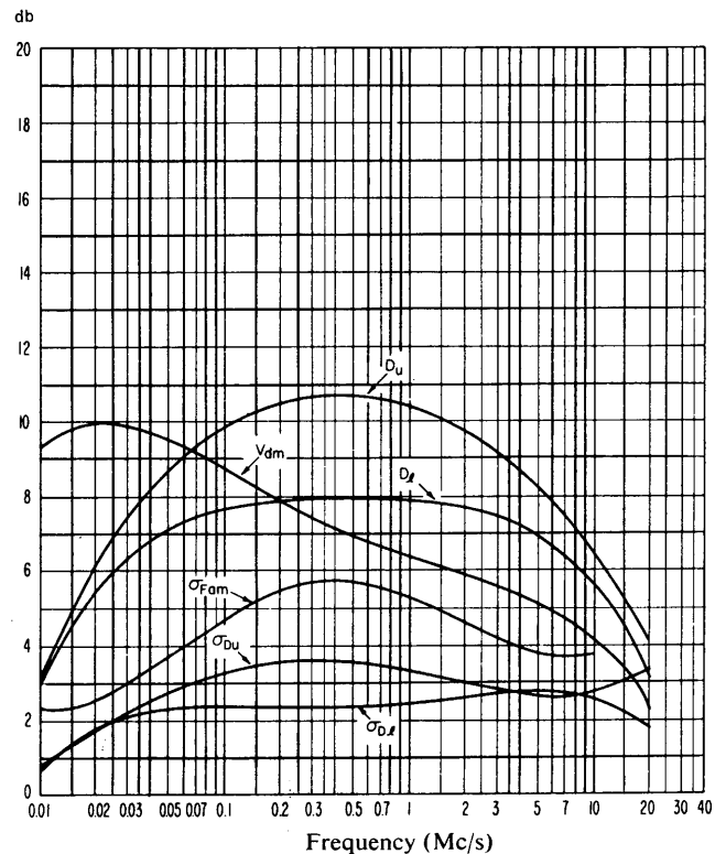
FIGURE 7C Data on noise variability and character (Winter; 2000–2400 h.)
