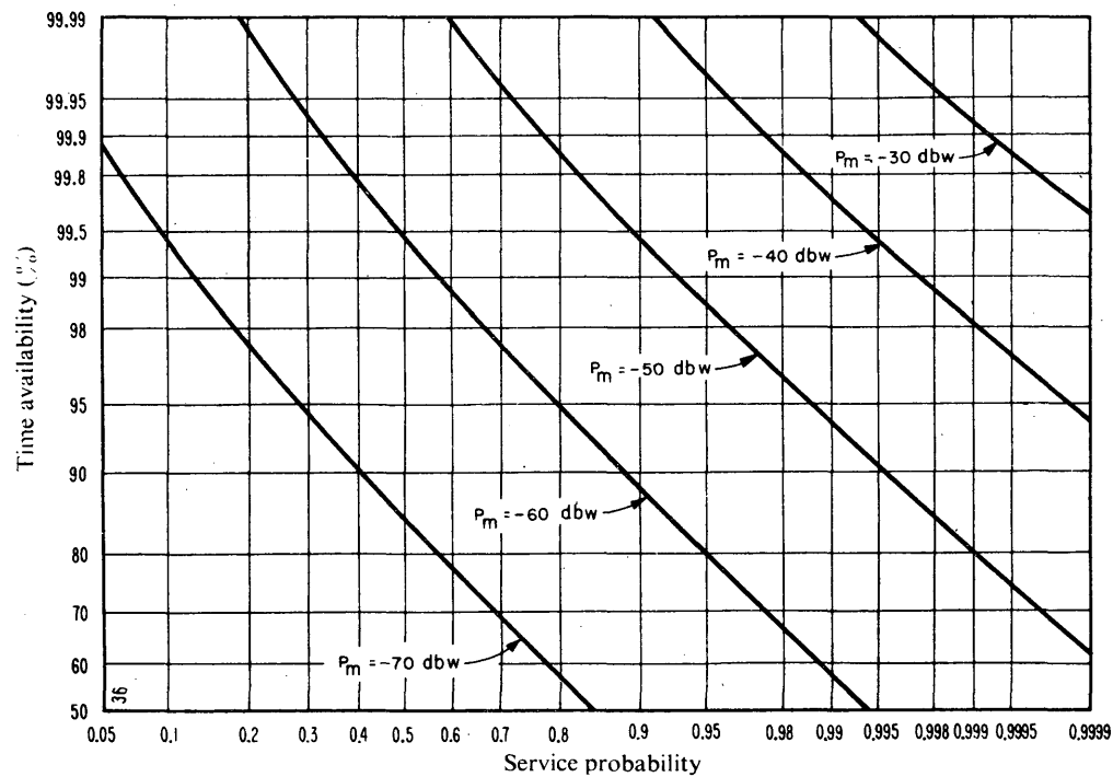
FIGURE 36 Time availability as a function of service probability Geneva, Switzerland Summer season, 2000–2400 h. Frequency: 5 Mc/s Bandwidth: 6 kc/s A3 telephony, marginally commercial service
