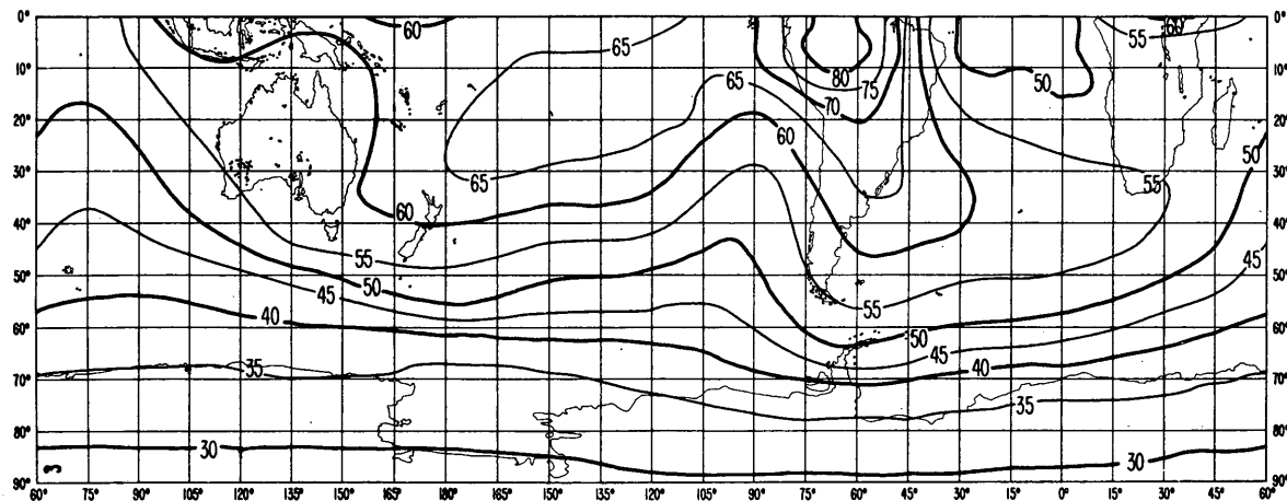
FIGURE 3A Expected values of atmospheric radio noise, F_{am} , (db above kT_0b at 1 Mc/s) (Winter; 0400-0800 h.)
