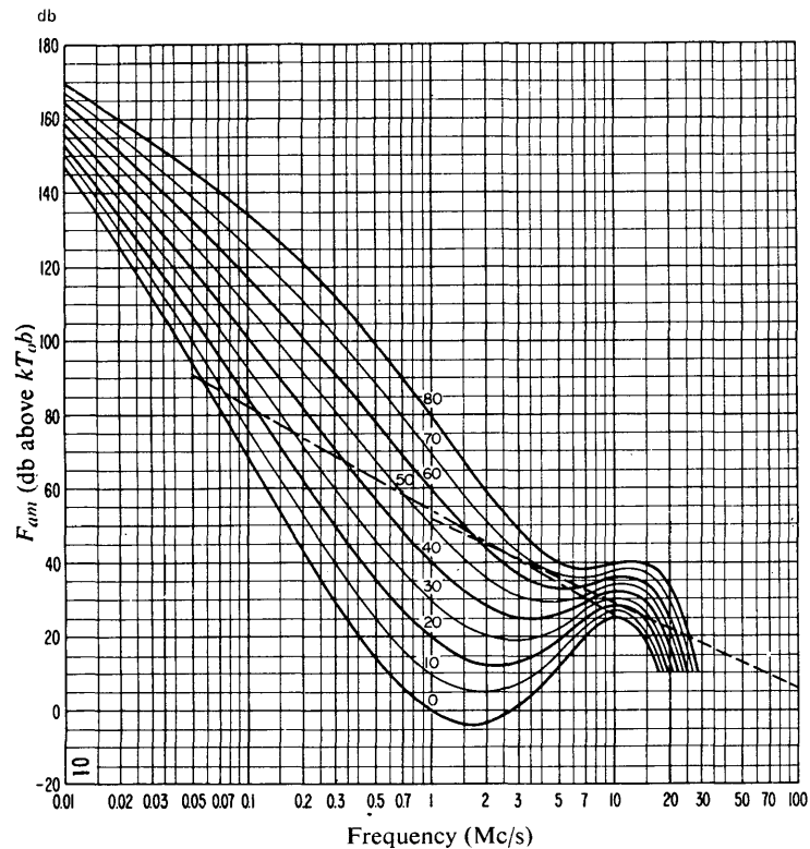
FIGURE 10B Variation of radio noise with frequency (Spring; 0800-1200 h.)
