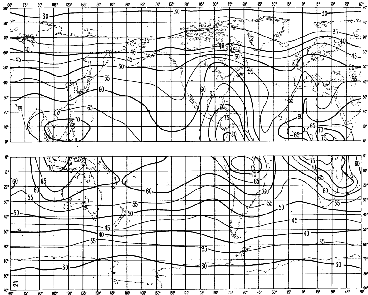
FIGURE 21A Expected values of atmospheric radio noise, F_{am} , (db above kT_b at 1 Mc/s) (Autumn; 0400-0800 h.)
