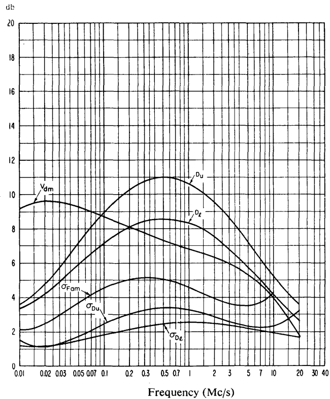
FIGURE 2C Data on noise variability and character (Winter; 0000-0400 h.)
