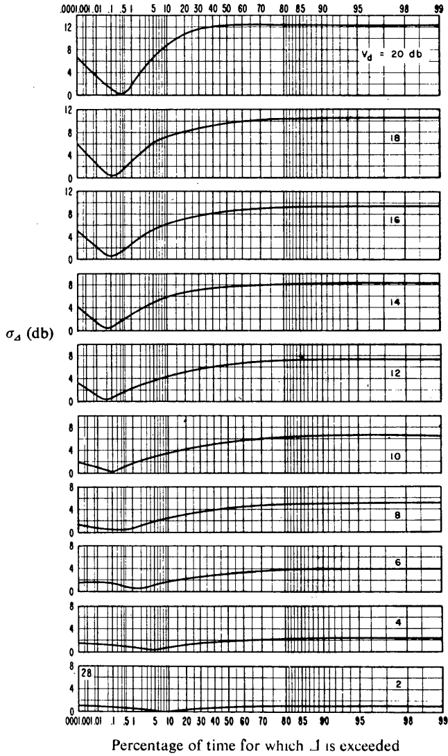
FIGURE 28 Standard deviations, \sigma_A
