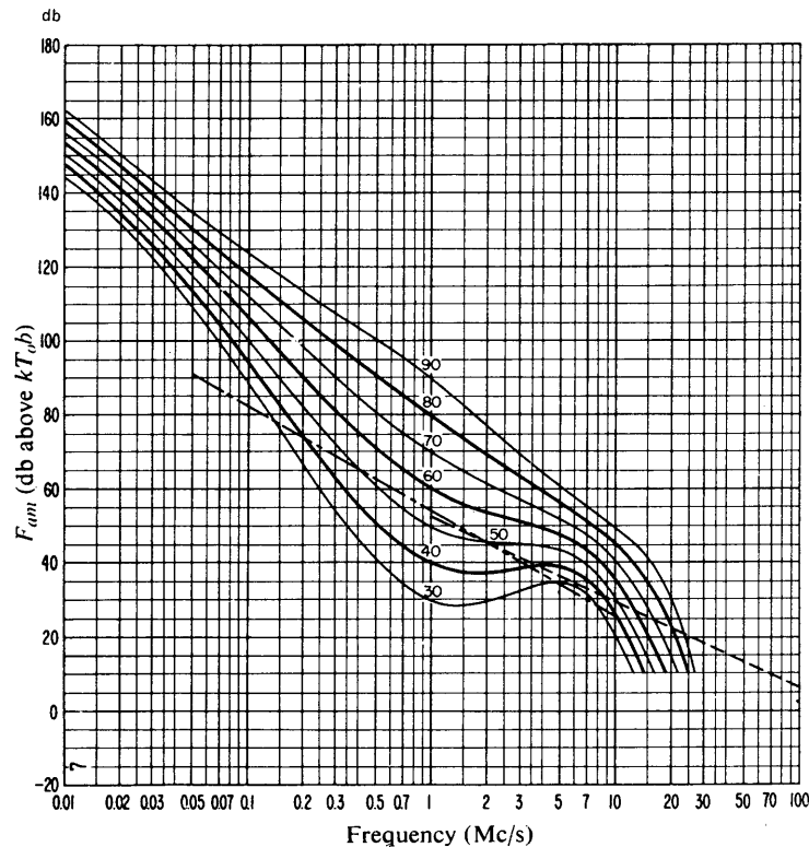
FIGURE 7B Variation of radio noise with frequency (Winter; 2000–2400 h.)
