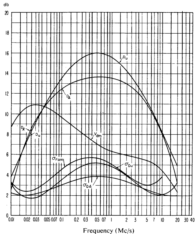
FIGURE 9C Data on noise variability and character (Spring; 0400-0800 h.)
