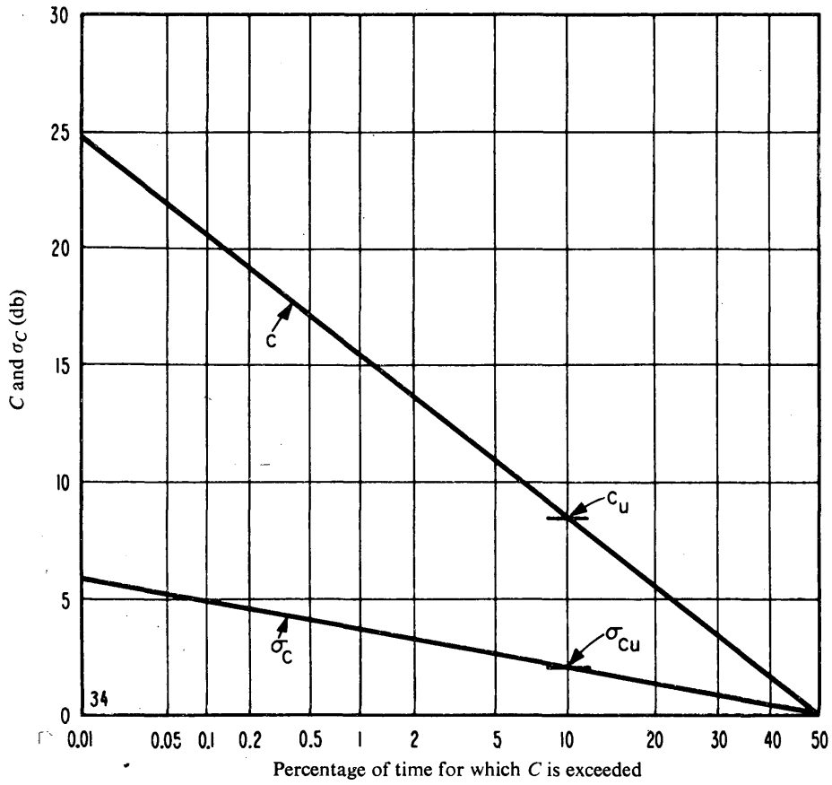
FIGURE 34 Expected values of C and their standard deviation, \sigma_C Summer season, 2000–2400 h. Frequency: 5 Mc/s
