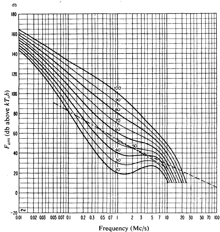
FIGURE 2B Variation of radio noise with frequency (Winter; 0000-0400 h.)
