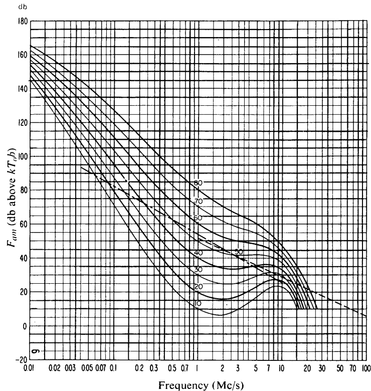
FIGURE 9B Variation of radio noise with frequency (Spring; 0400-0800 h.)
