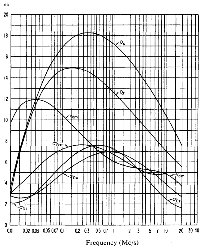
FIGURE 11C Data on noise variability and character (Spring; 1200–1500 h.)
