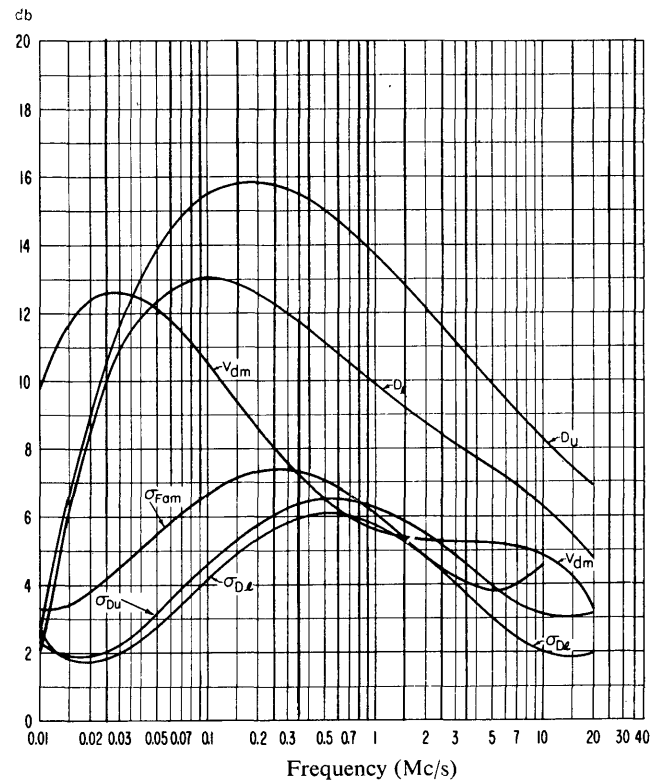
FIGURE 10C Data on noise variability and character (Spring; 0800-1200 h.)
