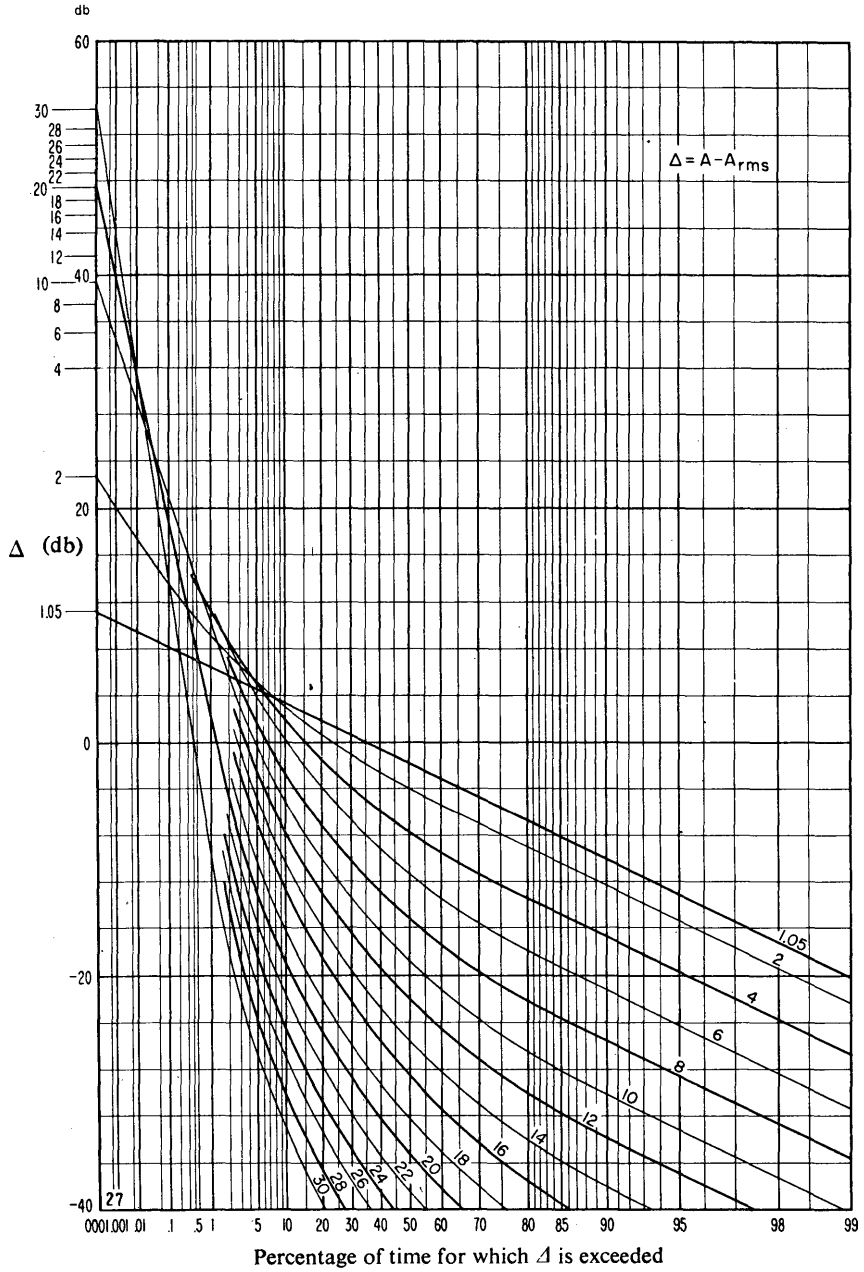
FIGURE 27 Amplitude probability distribution of the noise envelope
